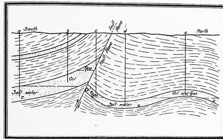
NO. 28. FAULT STRUCTURE AND OTHER OIL POSSIBILITIES.
