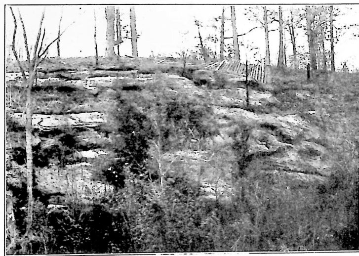
NO. 11. WEATHERING OF CASEVILLE CONGLOMERATE.
