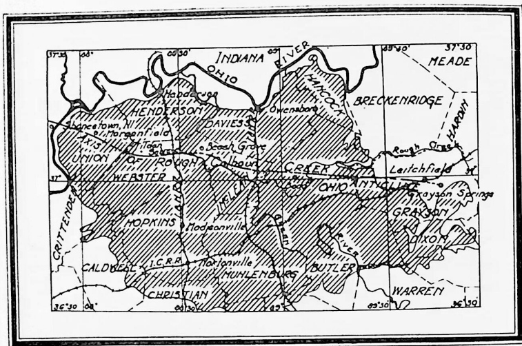
NO. 1. SKETCH MAP OF WESTERN KENTUCKY COAL FIELD.
