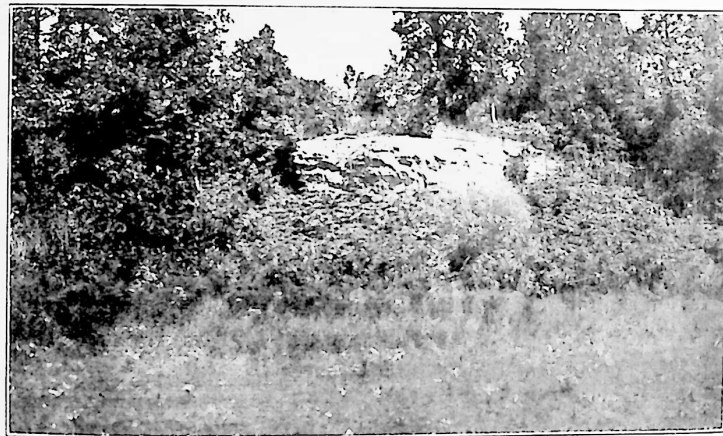
NO. 15. TOP OF CASEYVILLE CONGLOMERATE.
