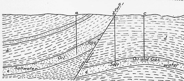
NO. 27. FAULT STRUCTURE AND OIL POSSIBILITIES.
