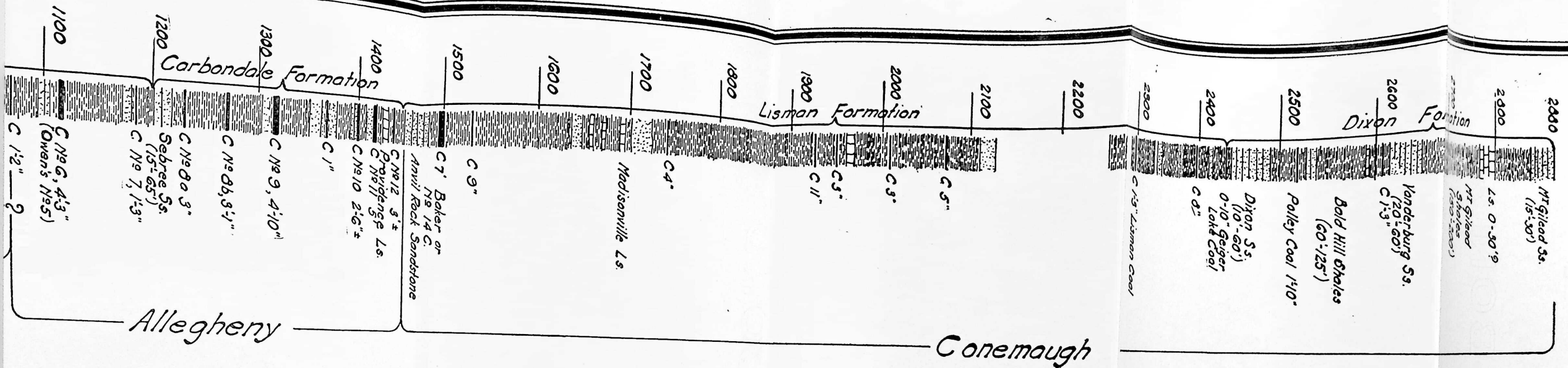
Plate XXXI Generalized Vertical Section of PENNSYLVANIAN Rocks to accompany report on the GEOLOGY AND COALS of WEBSTER COUNTY KENTUCKY by L.C. Glenn
