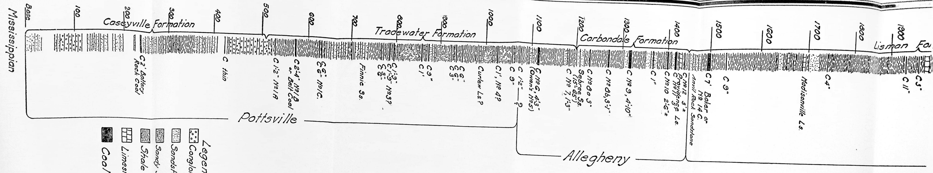
Plate XXXI Generalized Vertical Section of PENNSYLVANIAN Rocks to accompany report on the GEOLOGY AND COALS of WEBSTER COUNTY KENTUCKY by L.C. Glenn
