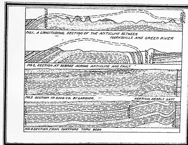
NO. 23. VERTICAL STRUCTURE SECTIONS.
