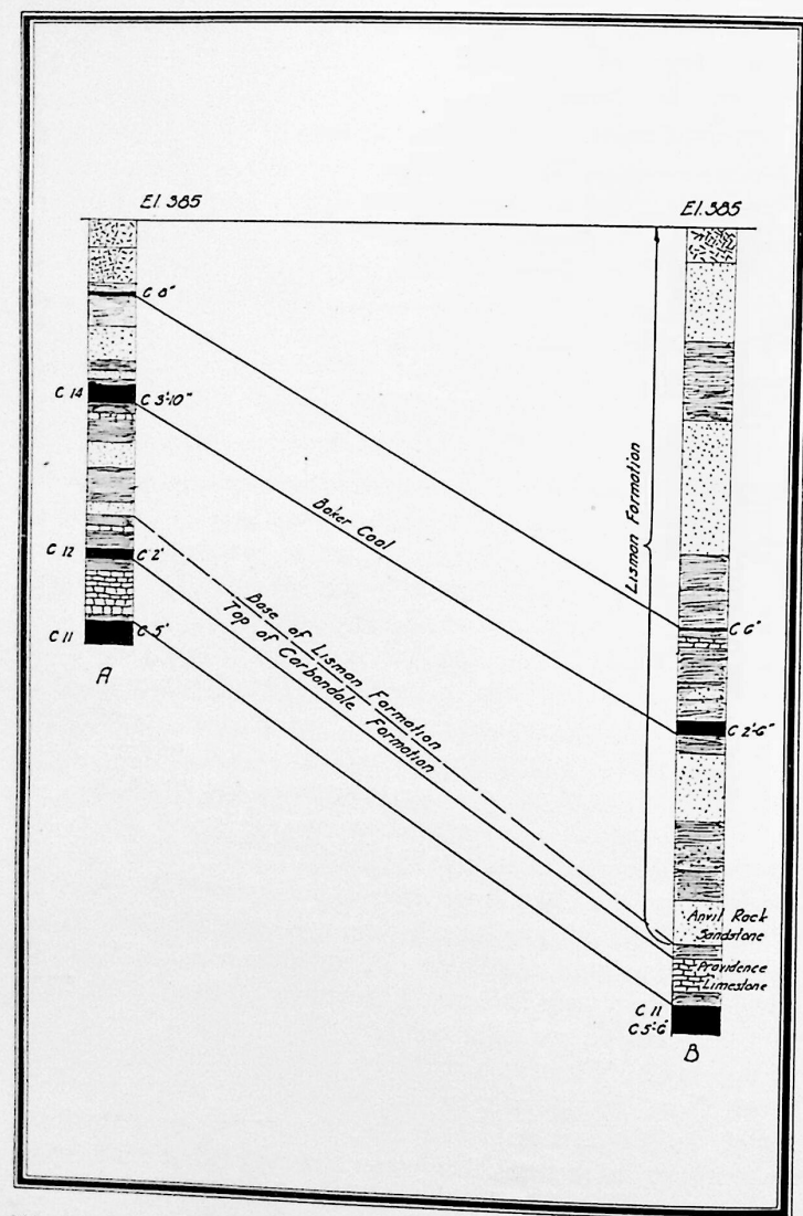
NO. 20. DETAILED SECTIONS ABOVE COAL NO. 11, WHEATCROFT.
