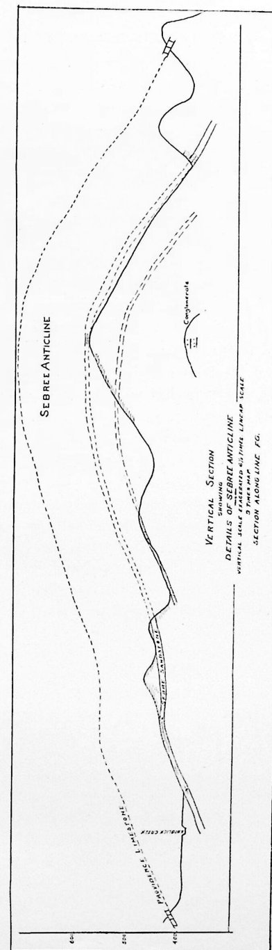
NO. 24. SECTION OF THE SEBREE ANTICLINE.
