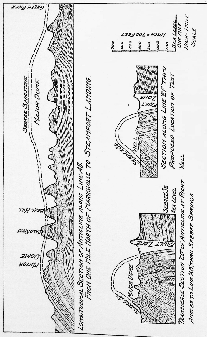
NO. 22. VARIOUS STRUCTURE SECTIONS IN WEBSTER COUNTY.
