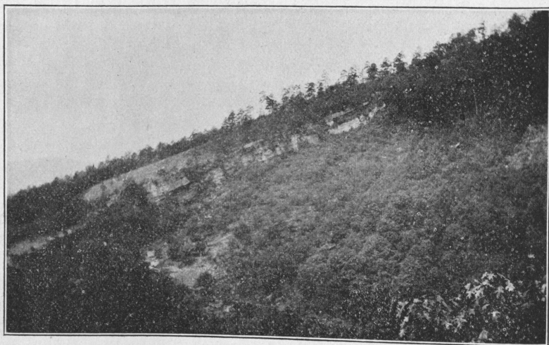
THE MOUNTAIN MAKING POTTSVILLE.
