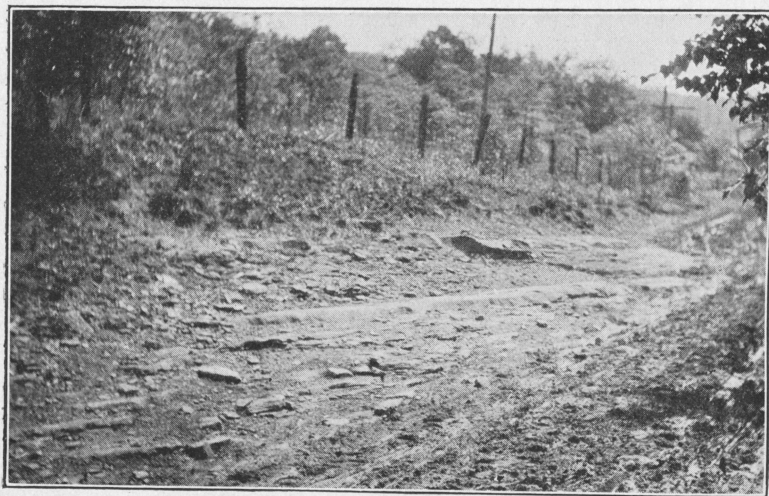
NORTHEAST FLANK OF ARTEMUS DOME.
