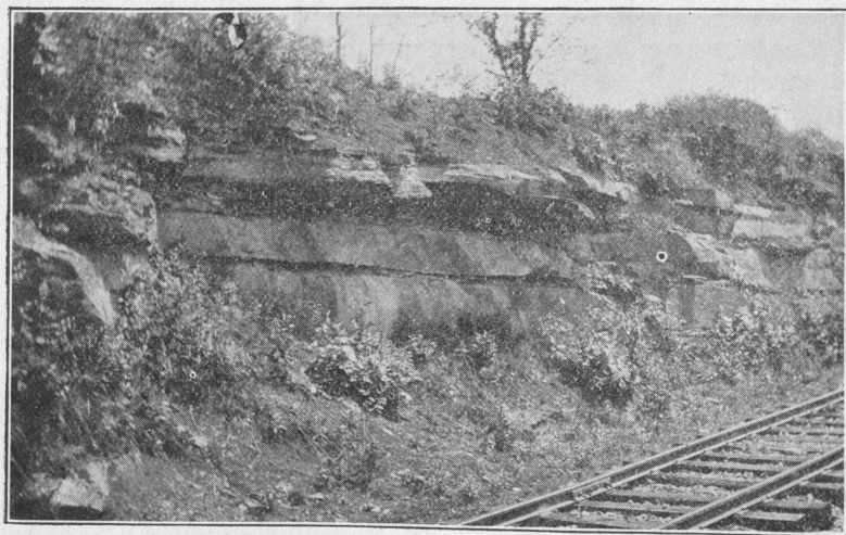
CREST OF ARTEMUS DOME.
