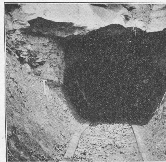
SMALL OPENING IN BLUE-GEM.
