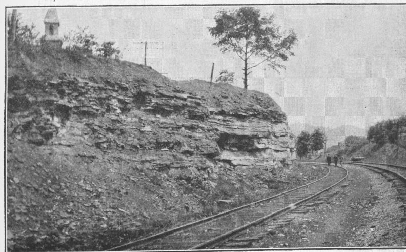
POTTSVILLE SANDSTONE NEAR ARTEMUS.
