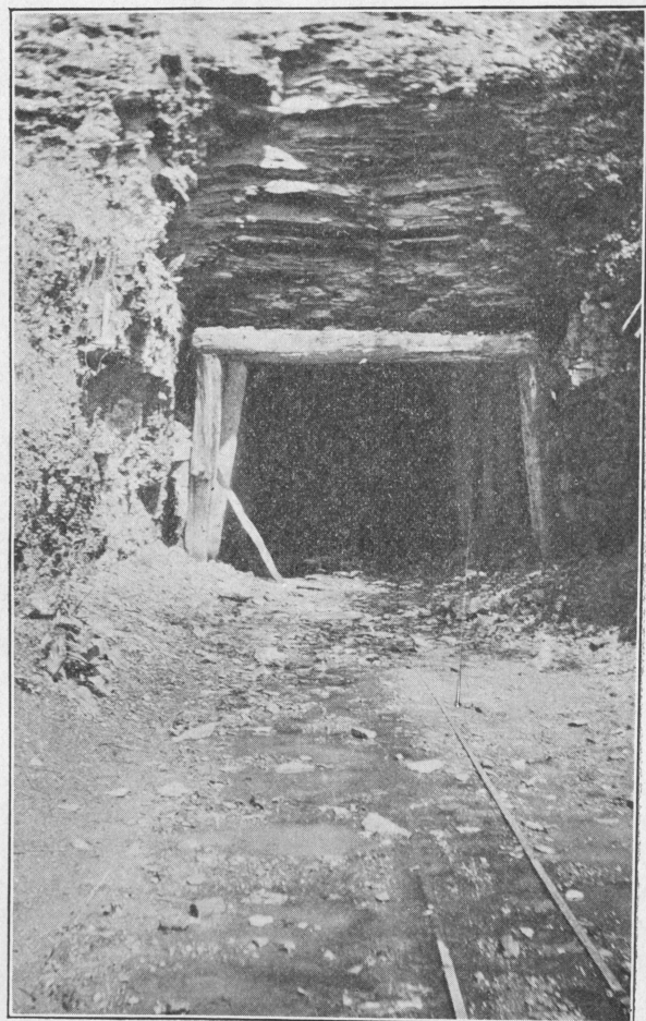
A BARBOURVILLE BLUE-GEM ENTRY.
