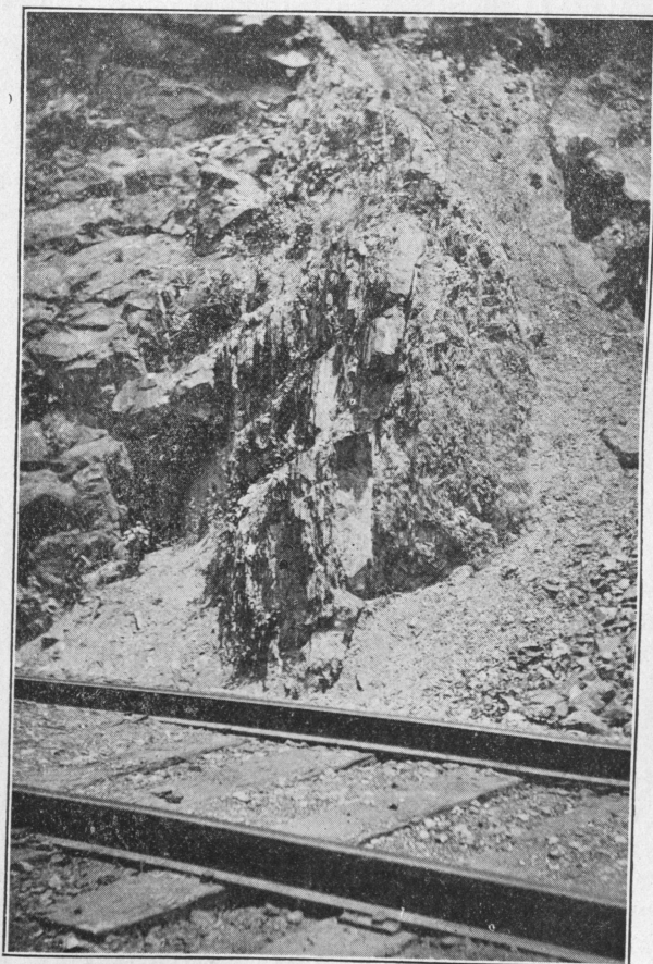
NEARLY VERTICAL BEDS—PINE MOUNTAIN FAULT. View in Louisville & Nashville Railroad cut just southeast of the mouth of Straight Creek. Photo by W. R. Jillson, May 16, 1919.
