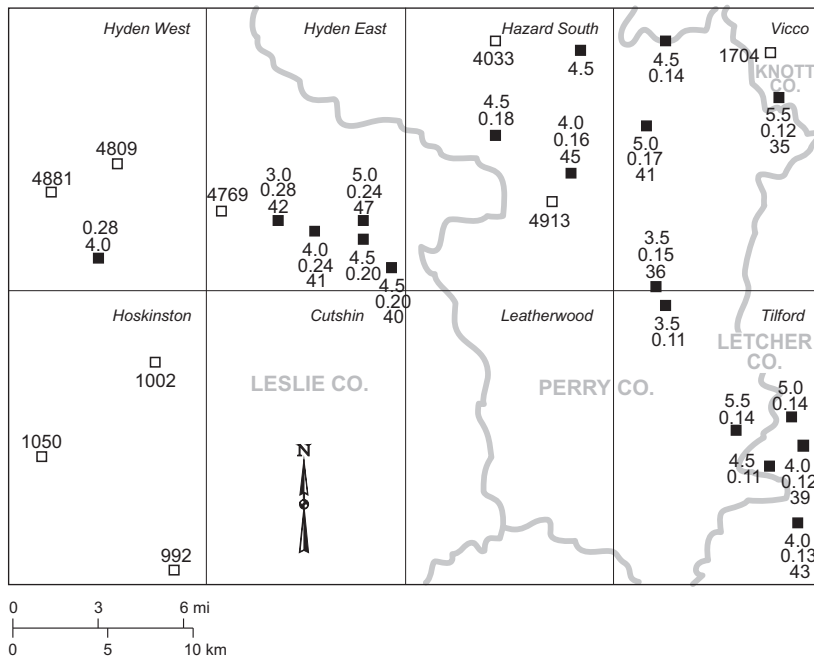
Lepidophloios ), and L. pusilla (produced by Lepidodendron ) are generally the most abundant species. Lycospora micropapillata and L. orbicula (both produced by Paralycopodites ) are locally abundant. In contrast, the lower bench tends to be more diverse in composition, with spores of small lycopsids (mostly Densosporites ), ferns (tree-like forms such as Punctatisporites minutus and Apiculatasporites saetiger , and small varieties such as Granulatisporites ), calamites ( Calamospora and large species of Laevigatosporites ), and cordaite pollen ( Florinites ) occurring more frequently.
