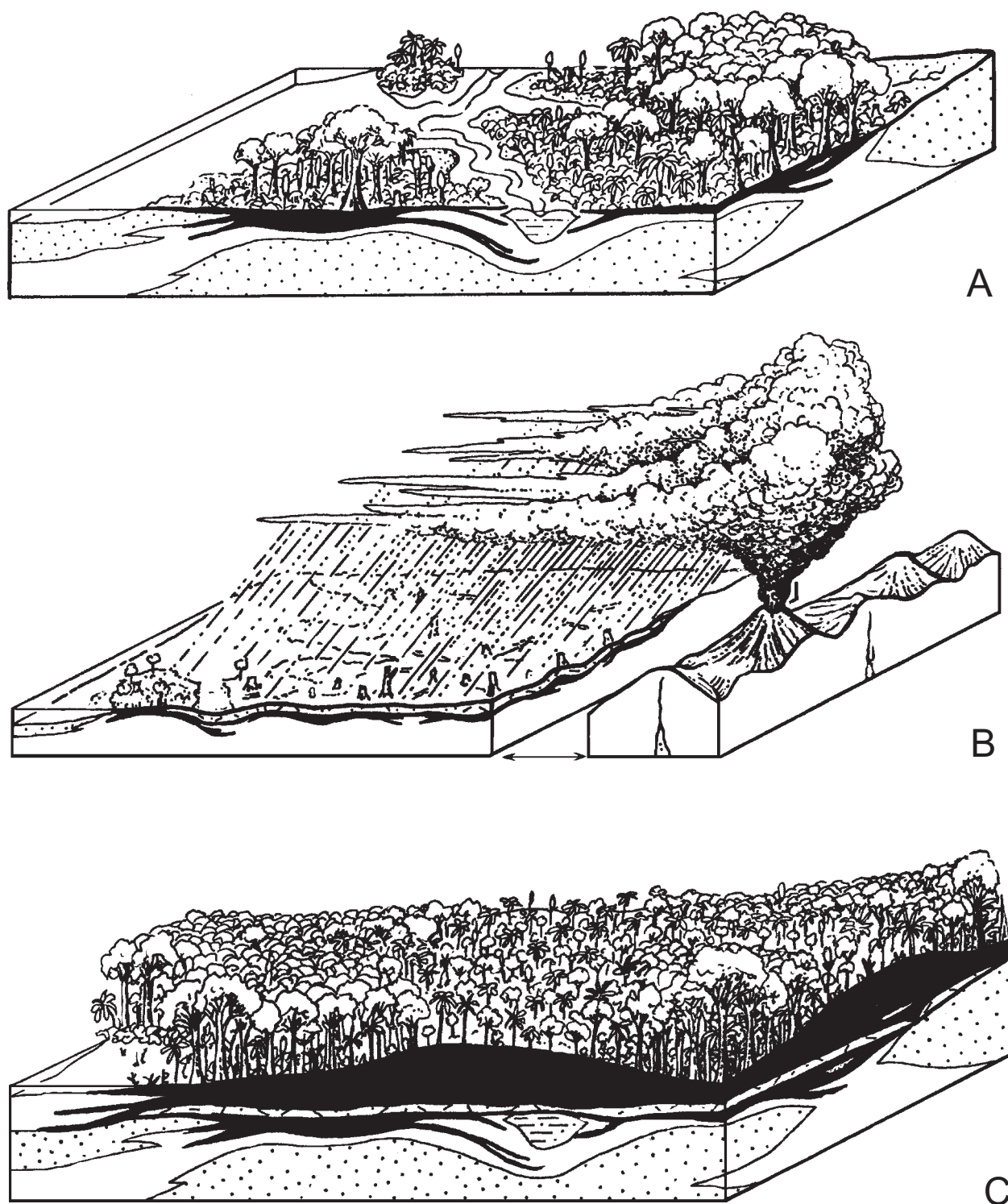
Figure 11. The evolution of the Fire Clay paleomire. (a) Peat started accumulating in a planar, rheotrophic mire that was discontinuous and subject to clastic influx. This peat is preserved as the lower bench of the Fire Clay coal bed. (b) Volcanic ash, which is ultimately preserved as a flint-clay parting, is deposited. (c) Peat accumulates after the ash fall and is preserved as the upper bench of the Fire Clay coal bed. Some parts of this bench are interpreted as having been derived from domed, ombrogenous peat.
