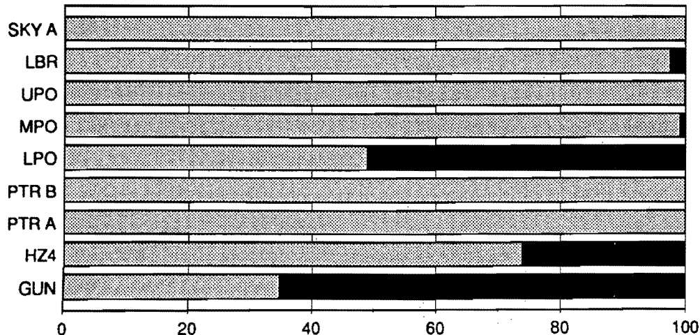
Figure 6. Percentages of original, remaining, and available coal resources in the 0-to-100-foot and 100-to-1,000-foot overburden categories. Abbreviations are explained in Figure 2.
