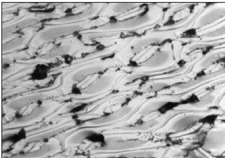
Coal is composed of macerals, which are analogous to minerals in a rock. This is a photomicrograph of the maceral semifusinite, which is wood or bark tissue oxidized by fire or microbial decay. Magnification 640X. Photo by Cortland Eble.
