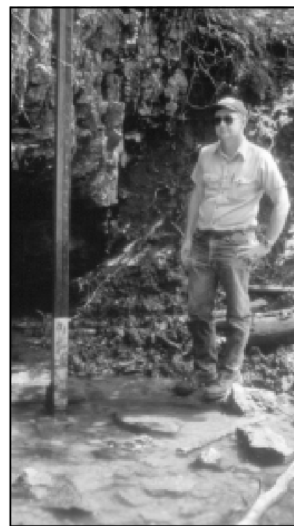
Stream flow is measured with a staff gage like the one in this photograph. Photo by James Cobb.
