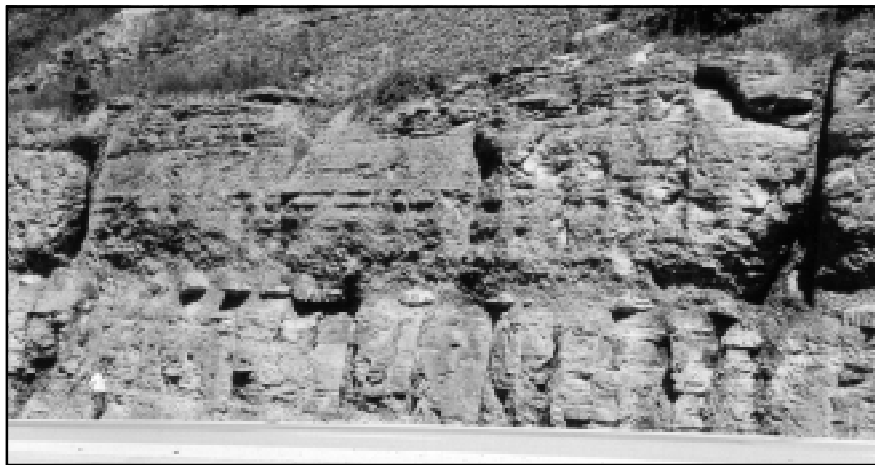
Fractures exposed at a roadcut along Kentucky 80, which were identified by lineament analysis. Photo by David Wunsch.
