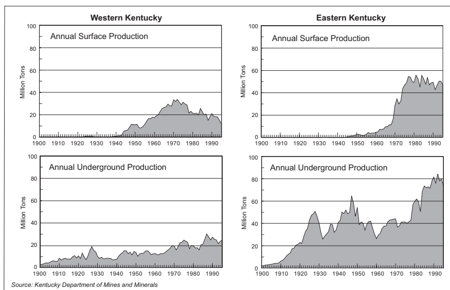
Annual production from 1900 to 1995 by coal field and mine type.
