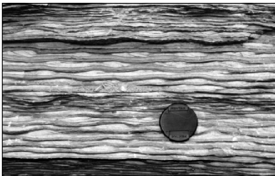
Rhythmically bedded strata that were deposited under tidal influences in an estuarine environment, called a tidalite, commonly occurs above coal beds in Kentucky. Photo by Cortland Eble.
