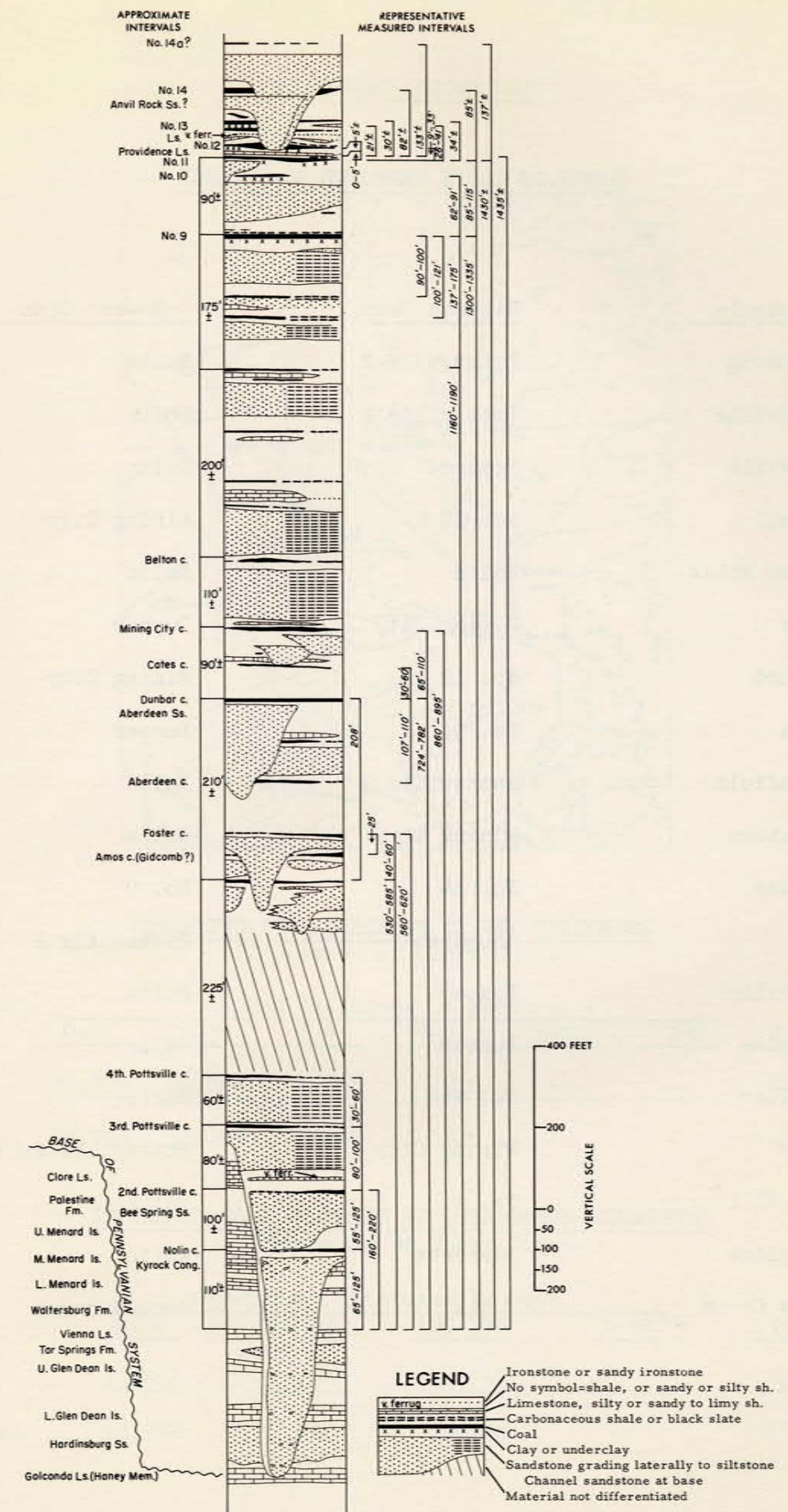
COMPOSITE STRATIGRAPHIC SECTION
