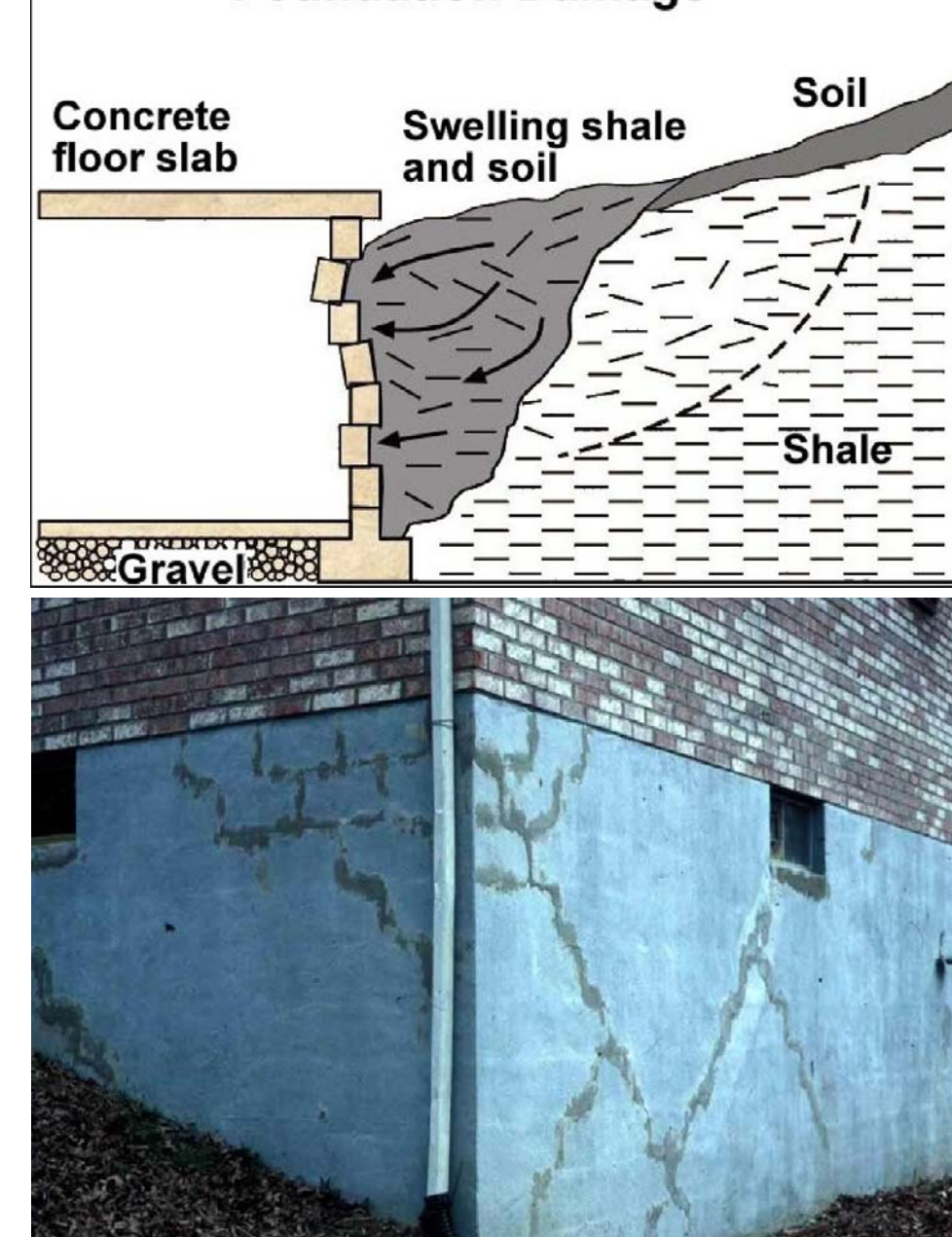
Some shales, and the soils derived from them, swell when exposed to water or air. These swelling shales and soils can have severe impacts on building foundations and other structures (e.g., bridges, dams, roads). Photo by John Kiefer, Kentucky Geological Survey.
