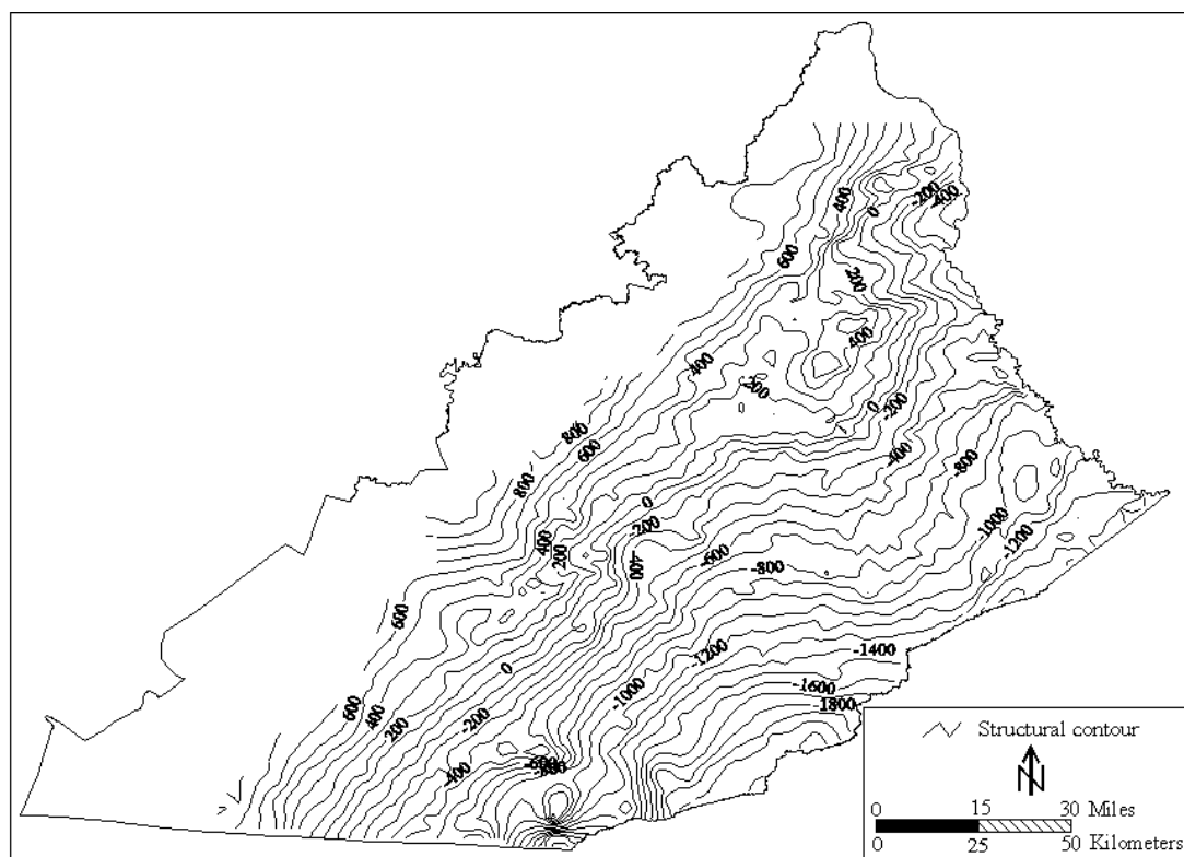
Figure 4.22: Regional structure contour map of the top of the Mississippian Newman Limestone. Contour interval equals 50 feet.
