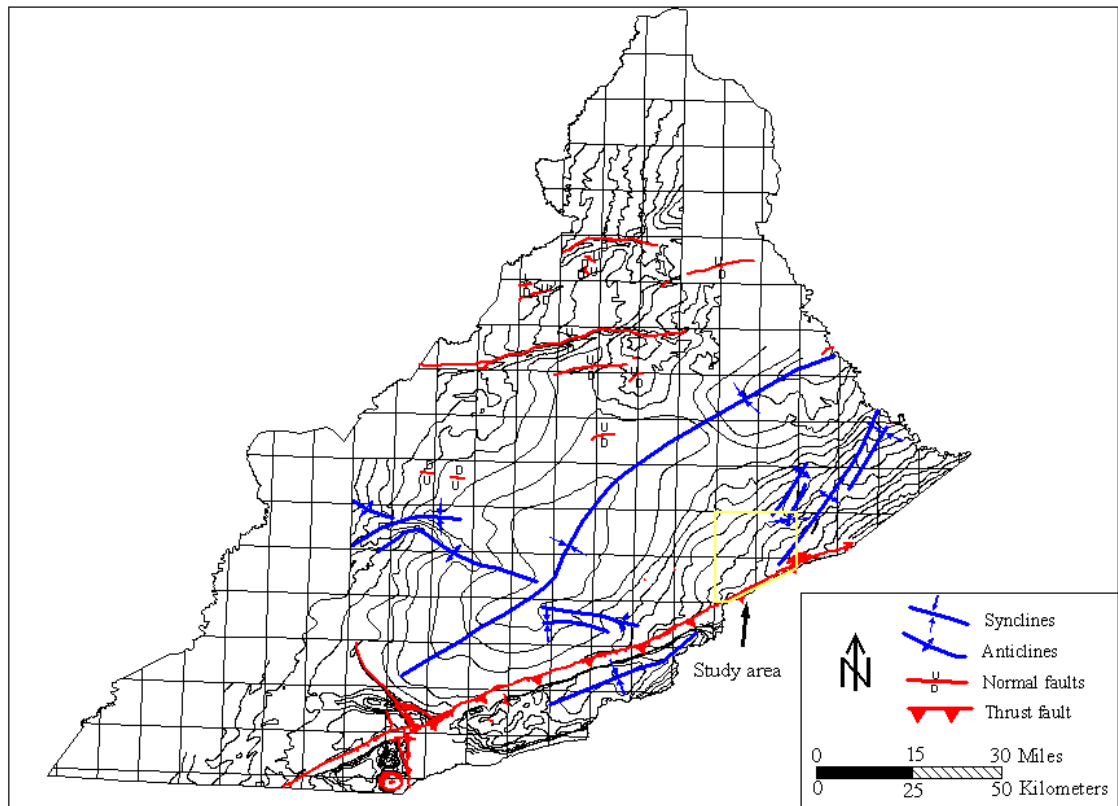
Figure 4.19: Regional structure map of the Lower Elkhorn coal showing the location of geologic structures. The four-quadrangle study area is highlighted in yellow.
