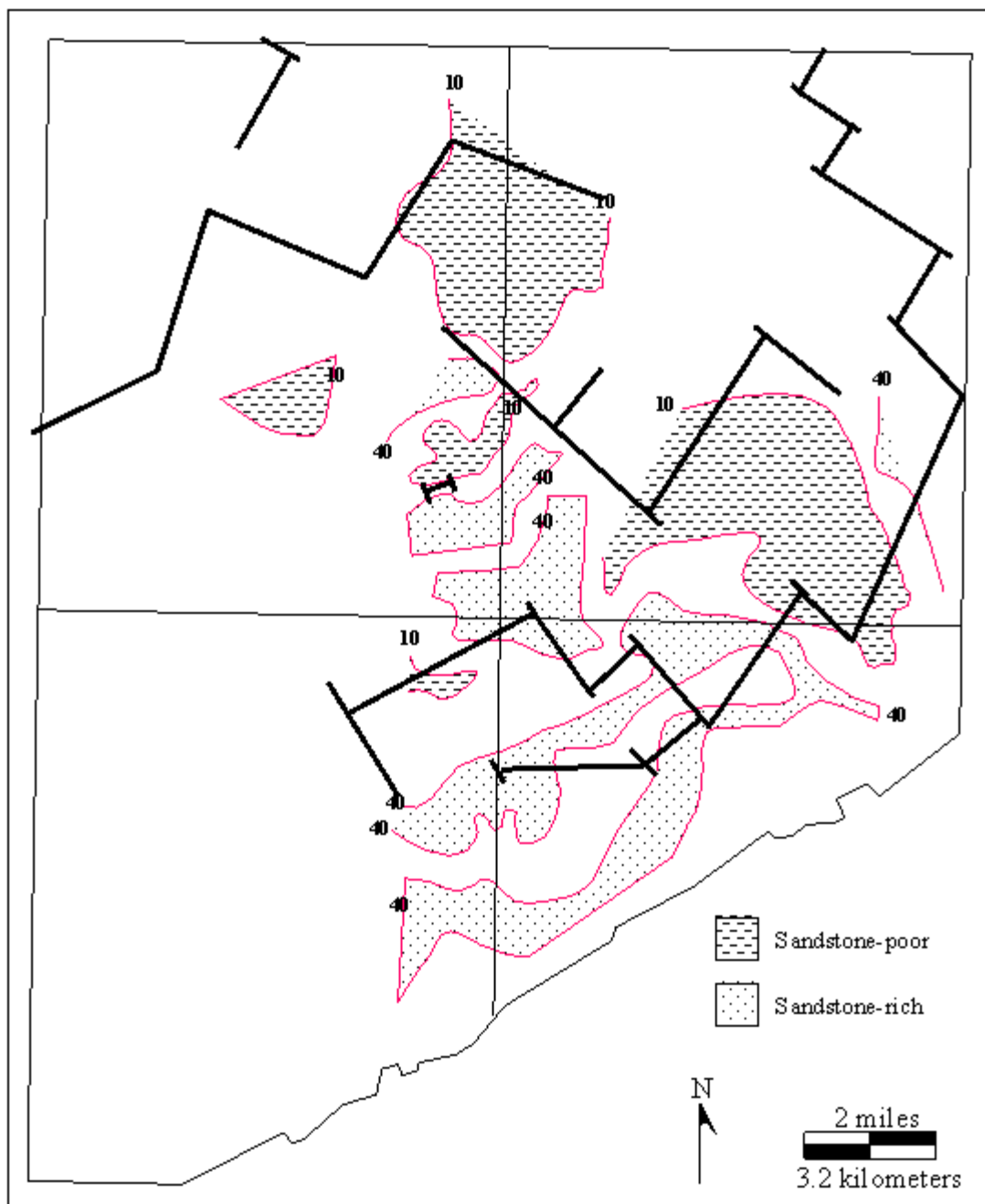
Figure 4.32: Lower Elkhorn/Elkhorn rider interval total sandstone isolith map showing the relationship between sandstone-rich and sandstone-poor areas and inferred faults.
