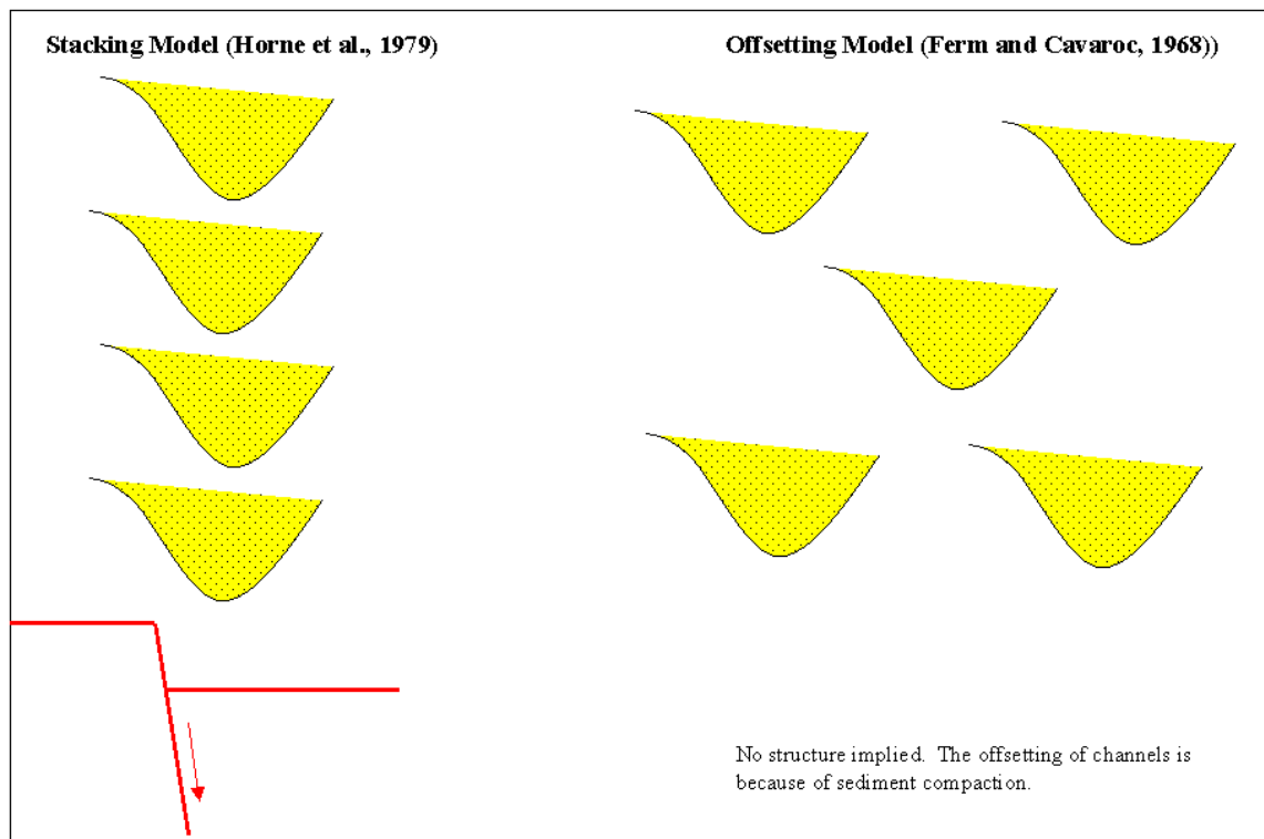
Figure 1.1: Generalized diagram showing the offsetting model (Ferm and Cavaroc, 1968) versus the stacking model (Horne, 1979).
