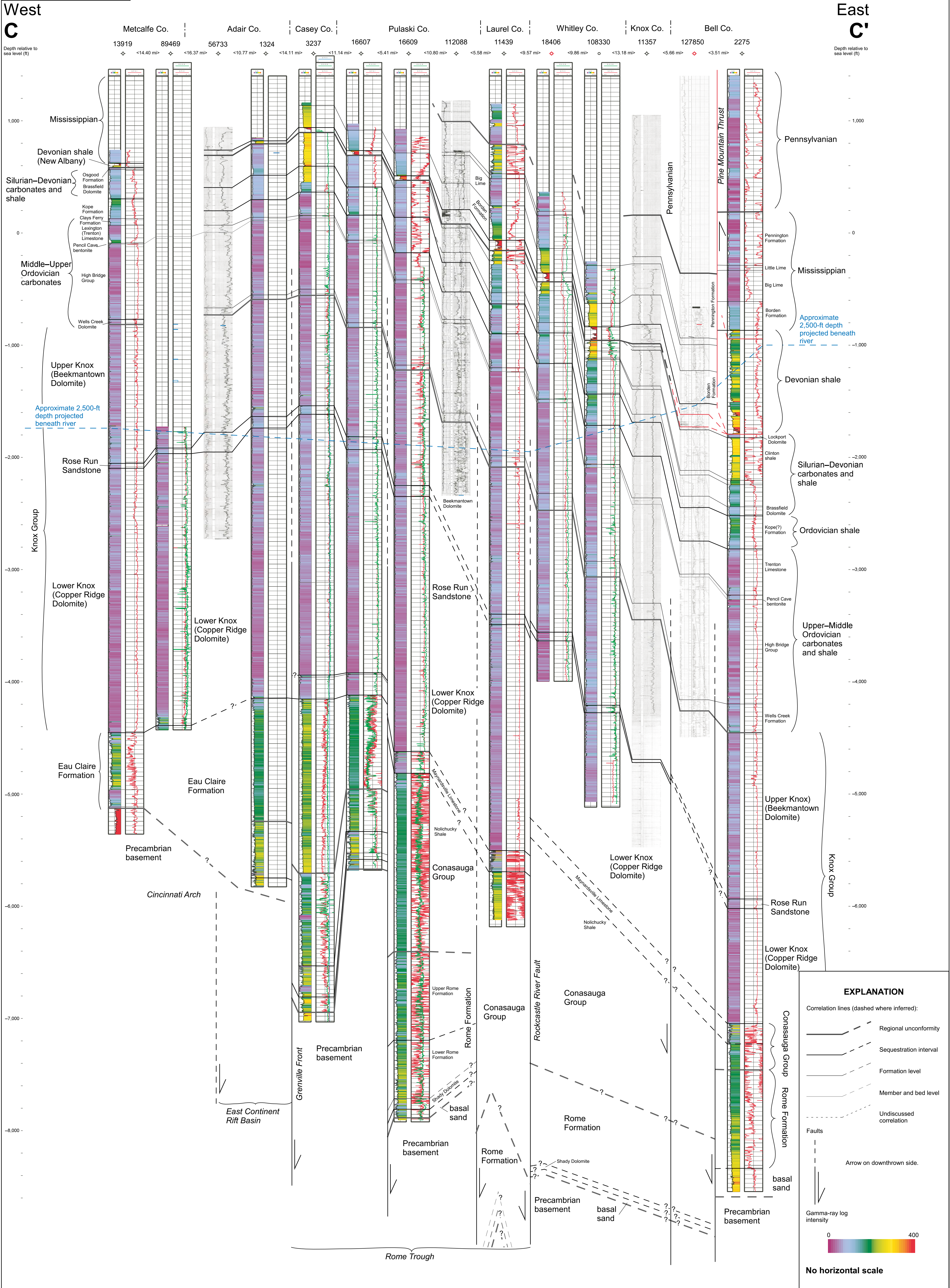
Plate 4.6. Cumberland River cross section. Chapter 4: Geologic Carbon Storage (Sequestration) Potential in Kentucky
