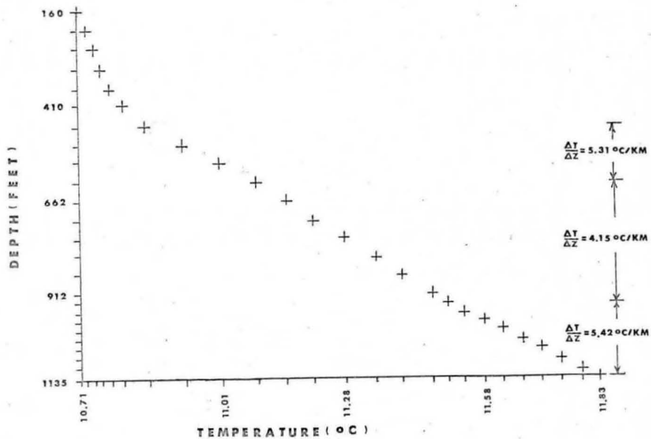
FIGURE 22 TEMPERATURE VS. DEPTH, HOLE CC-C, MARCH 28, 1969
