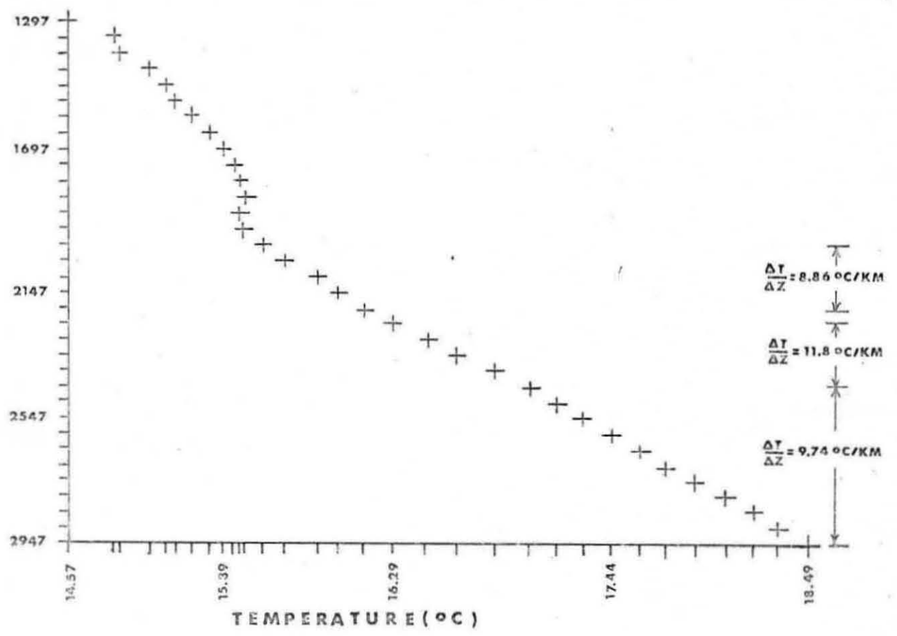
FIGURE 25 TEMPERATURE VS. DEPTH, HOLE CC-E, MAY 1, 1969
