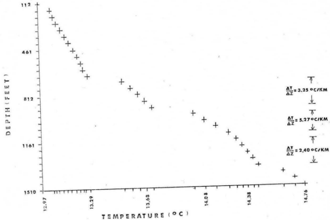
FIGURE 23 TEMPERATURE VS. DEPTH, HOLE CC-D, MARCH 21, 1969
