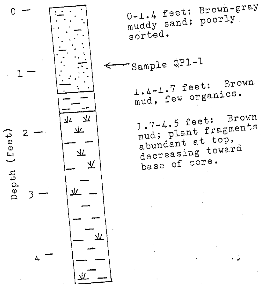
Figure 14a. Core log QP1-82. See Appendix for detailed sediment analysis.
