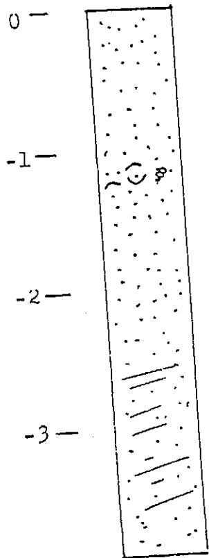
Figure 14c. Core log QP3-82. See Appendix for detailed sediment analysis.
