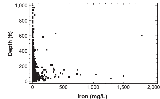
Figure 4. Plot of iron concentrations versus well depth.
