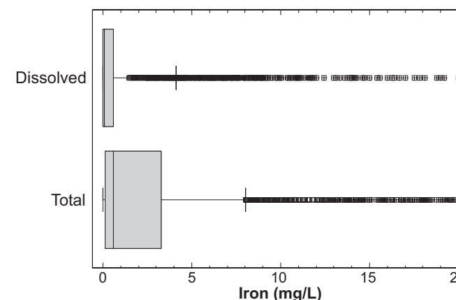
Figure 2. Comparison of total and dissolved iron concentrations. Higher values were excluded to better show the majority of the data.
