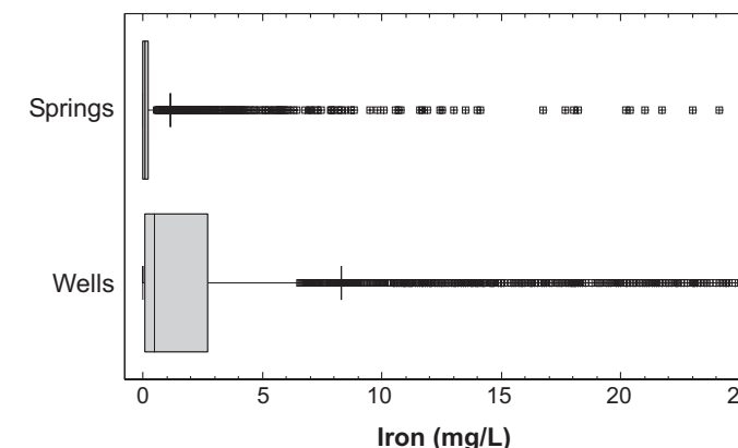
Figure 3. Comparison of iron concentrations in water from wells and springs. Higher values were excluded to better show the majority of the data.
