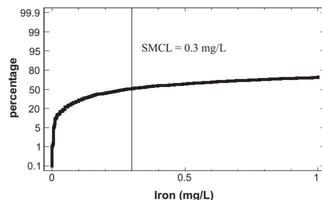
Figure 1. Cumulative percentage plot of measured iron concentrations. Higher values were excluded to better show the region of interest.
