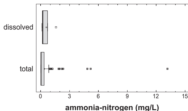
Figure 81. Comparison of total and dissolved ammonia-nitrogen concentrations. DOW recommendation=0.11 mg/L.
