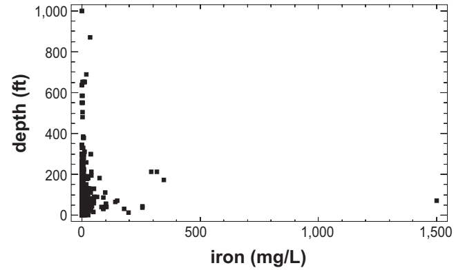
Figure 59. Iron concentrations versus well depth. SMCL=0.3 mg/L.
