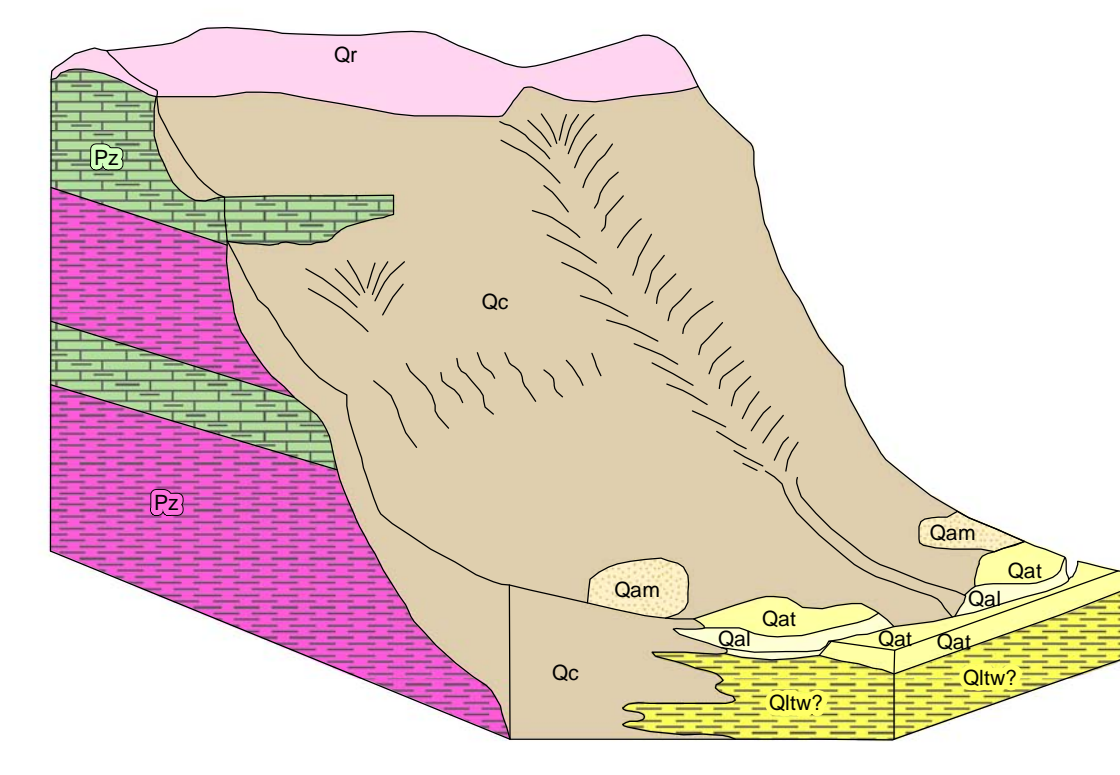
Figure 2. General diagrammatic model of the surficial deposits and geomorphology of part of the Alexandria quadrangle. Residual soil and colluvium mantle the hillsides and glacial lacustrine?, alluvium, and terrace deposits occupy the valleys. The green color Pz represents stratigraphy that contains more limestone and the purple more shale Modified from Wysocki and others, 2000 and Crawford, 2011.
