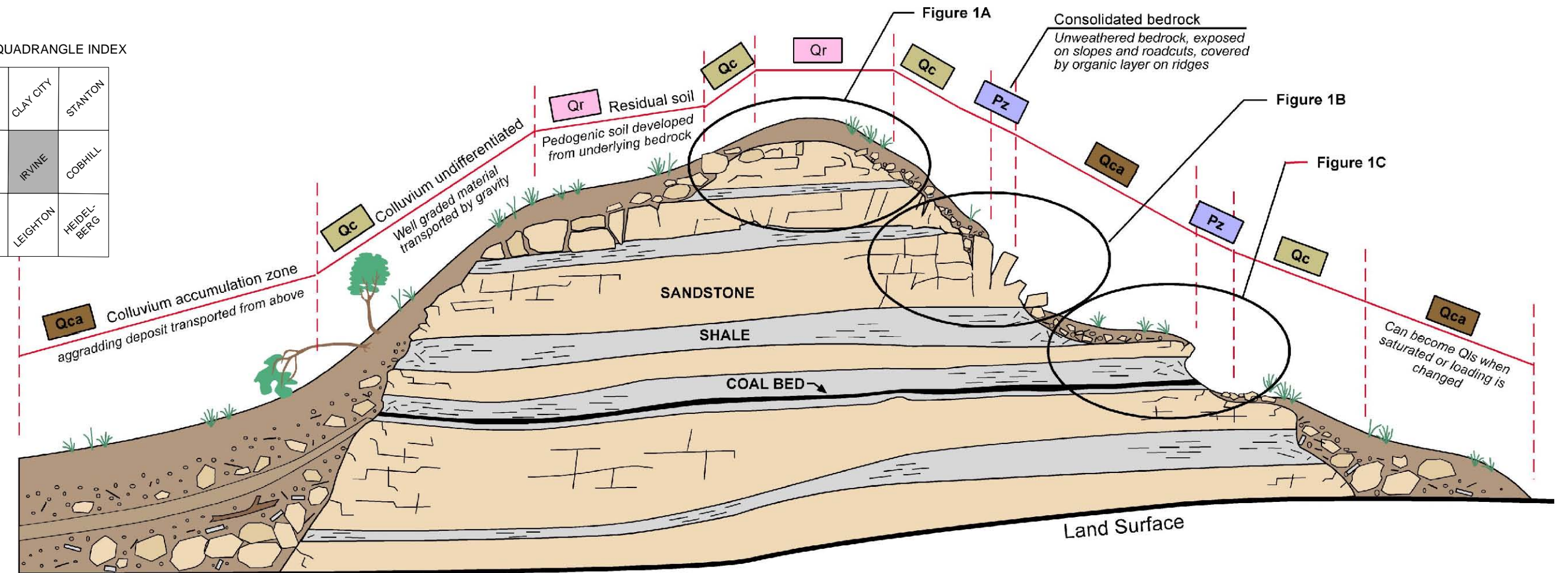
Figure 1. Conceptual model of the geomorphic processes in the Irvine 7.5-minute quadrangle
