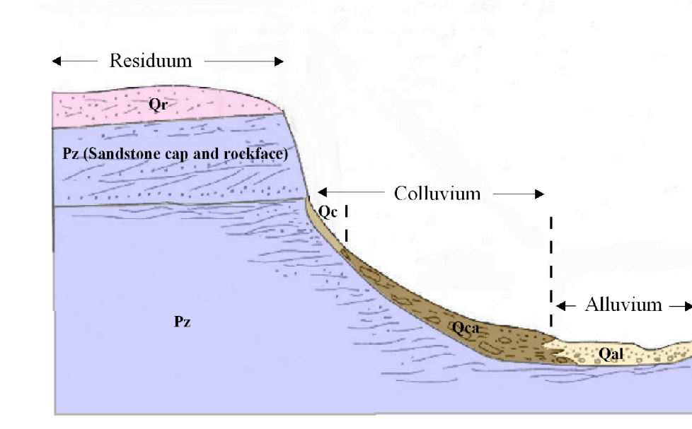
Figure B. Idealized cross-section of hillslope and surficial units formed on bedrock with a sandstone cap and vertical sandstone rock face. Note the difference in colluvium (Qc) and the colluvial accumulation zones (Qca). Here the Qca intersects a broader channel occupied by Qal. (Modified from Newell, 1978).
